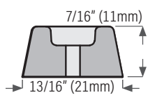
KT123 Bumper stop, attach with screw
