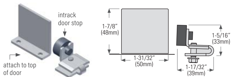
KT129 intrack door stop set for KT41 Series, KT51 Series
