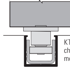
KT127SS2 Bottom guide, single roller (stainless steel) for floor channel or bottom door channel
