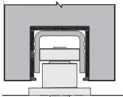
KT127SS1 Bottom guide, single roller (stainless steel) for floor channel or bottom door channel
